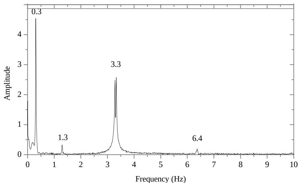
Figure 3-15. Sample of FFT
