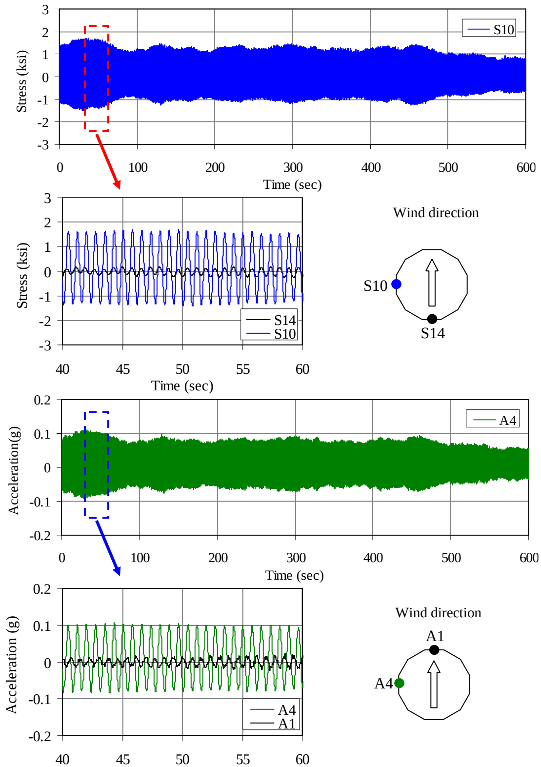
Figure 3-27. (Continued) Time (sec)
