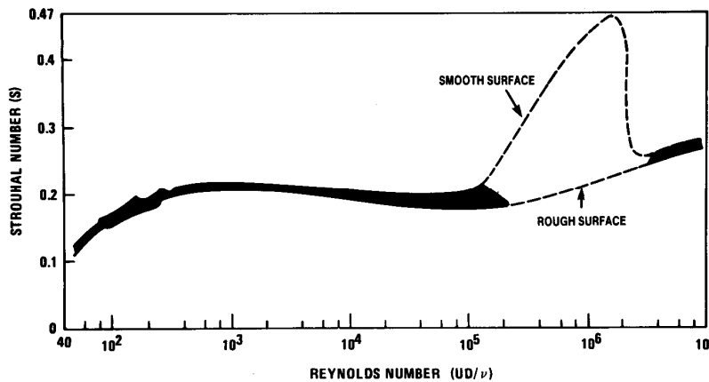
Figure 2-3. Strouhal number-Reynolds number relationship for circular cylinders
