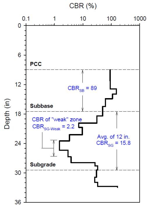
Figure 13. CBR profile
