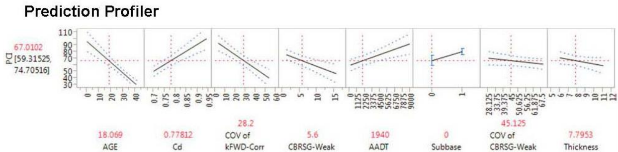
Figure 18. IHRB TR-640 multivariate analysis (IHRB TR-640 Field Data Report)
