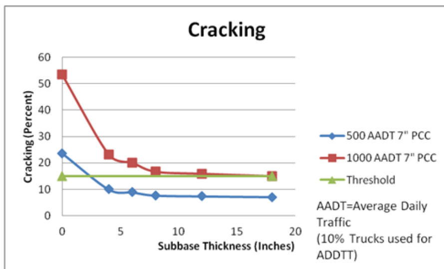
Figure 23. Cracking failure mode from Pavement ME Design
