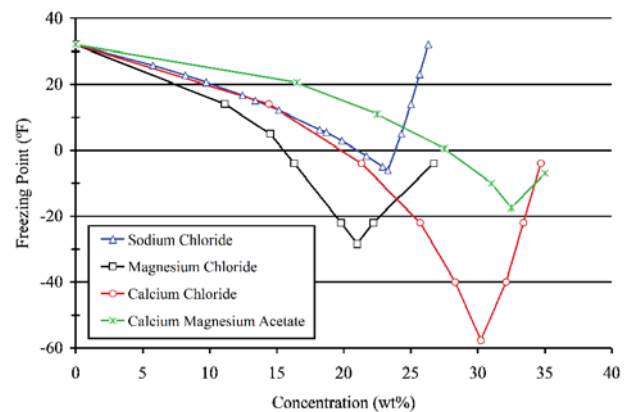
Figure 4-2. Partial phase diagrams for mixtures of water and common deicing/anti-icing salts. The freezing point of the water-salt solution (brine) is plotted as a function of the concentration of salt, in weight percent. Note that for all salts, a minimum freezing point is shown (Sutter 2008)
