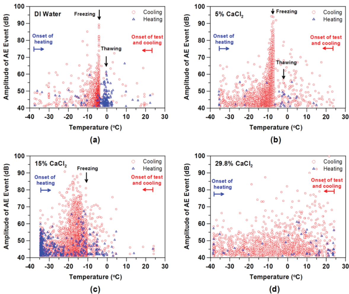
Figure 2-7. Passive AE events versus temperature during cooling and heating for mortar specimens saturated with (a) deionized water; (b) 5 percent \text{CaCl}_2 solution; (c) 15 percent \text{CaCl}_2 solution; and (d) 29.8 percent \text{CaCl}_2 solution (scattered AE activity can be seen for the 29.8 percent concentration)
