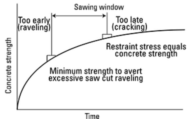
Figure 3-3. Sawing window
